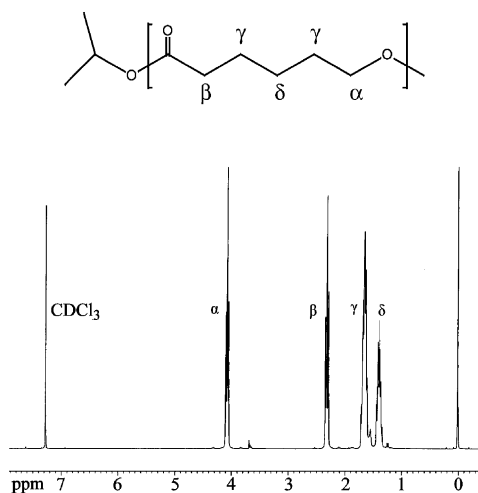
Fig. 3. 1 H NMR spectrum of PCL oligomer and its peak assignment.
