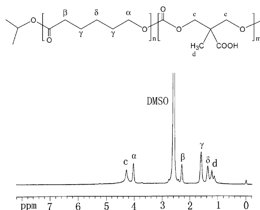
Fig. 5. 1 H NMR spectrum of PCL- b -PMCC1 and its peak assignment.
