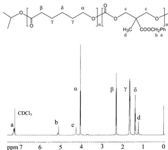
Fig. 4. 1 H NMR spectrum of PCL- b -PMBC1 and its peak assignment.
